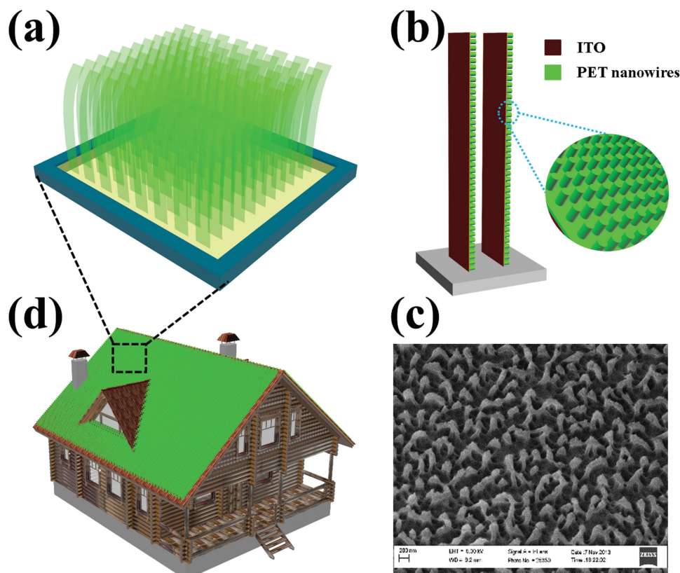
Figure 1. Lawn structured triboelectric nanogenerator. a) Schematical illustration of the TENG, which has a kelp-forest-like morphology. b) A basic unit of the TENG, which is a pair of strips, which is consisted of ITO coated PET with an end anchored onto the substrate and the other end stayed free-standing. c) SEM image of PET nanowires. d) A sketch shows that the TENG can be easily equipped to the rooftops for natural wind energy harvesting.
