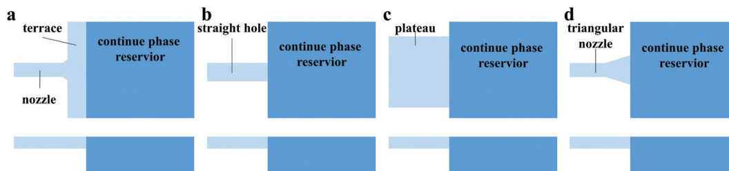
Fig. 2 Schematics of microfluidic step emulsification devices. (a) The grooved-type microchannel. (b) The straight-through microchannel. (c) The edge-based droplet generation (EDGE) device. (d) The triangular nozzle microchannel.
