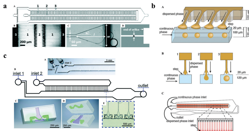
Fig. 6 Schematic of the triangular nozzle microchannel. (a) Schematic illustration of the millipede device with parallelized triangular nozzles. Reproduced from ref. 71 with permission from The Royal Society of Chemistry. (b) Layout and working principle of a glass microfluidic device for parallelized step emulsification. Reproduced from ref. 72 with permission from John Wiley and Sons. (c) Shunt channels modified triangular nozzle microchannel. Reproduced from ref. 74 with permission from The Royal Society of Chemistry.
