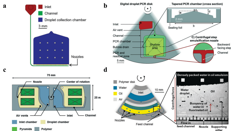
Fig. 8 Schematic of the centrifugal step emulsification. (a) Schematic of the centrifugal step emulsification with 23 parallel nozzles. Ref. 76 – Published by The Royal Society of Chemistry. (b) Schematic of the centrifugal step emulsification with a tapered reservoir for digital droplet PCR on disk. Ref. 78 – Published by The Royal Society of Chemistry. (c) Centrifugal DropChip for ddLAMP. Ref. 79 – Published by The Royal Society of Chemistry. (d) Centrifugal step emulsification with a tree-typed microchannel. 80 Published by MDPI.
