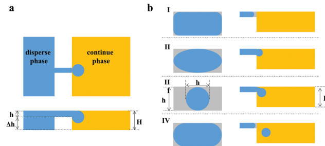
Fig. 1 Schematic of step emulsification. (a) Top and side views of the step emulsification structure. (b) Cross-sectional views of the nozzle in two lateral directions. I. The dispersed phase is injected into the nozzle; II. The radius of bulb reaches the critical value and begins to form the necking region; III. The diameter of the neck decreases to the nozzle height after necking; IV. The droplet detaches from the dispersed phase into the continuous phase.
