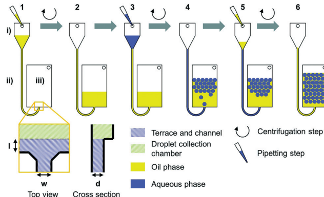
Fig. 7 Workflow of centrifugal step emulsification. The system is located on a spinning disk and consists of an inlet chamber (i), a channel (ii) which connects the inlet to a nozzle, and a droplet collection chamber (iii). Reproduced from ref. 76 with permission from The Royal Society of Chemistry.
